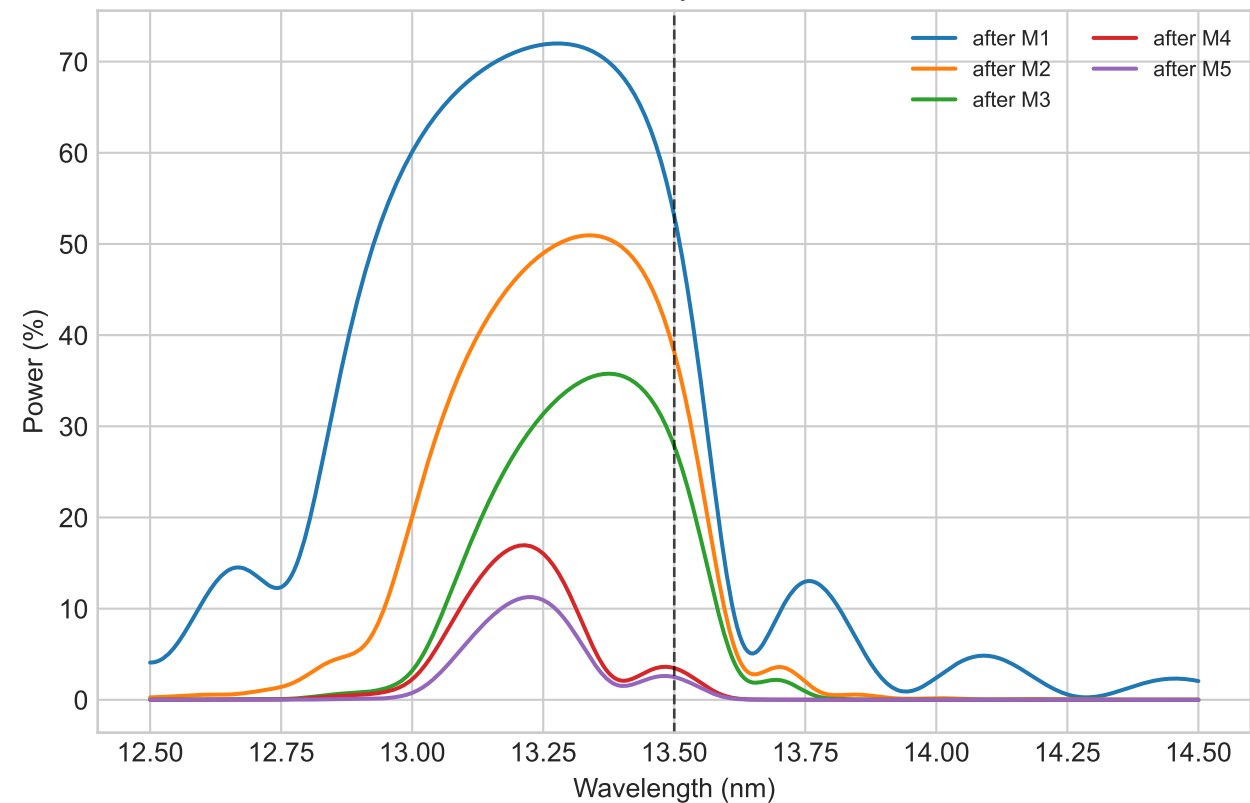
Cumulative intensity after each mirror
